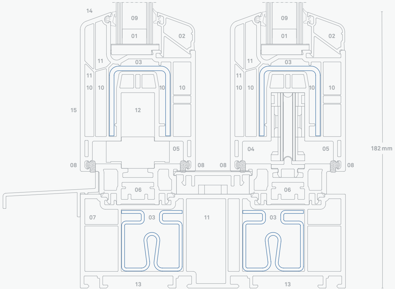
Inoutic HST 76 Prestige | 76.4 C2
